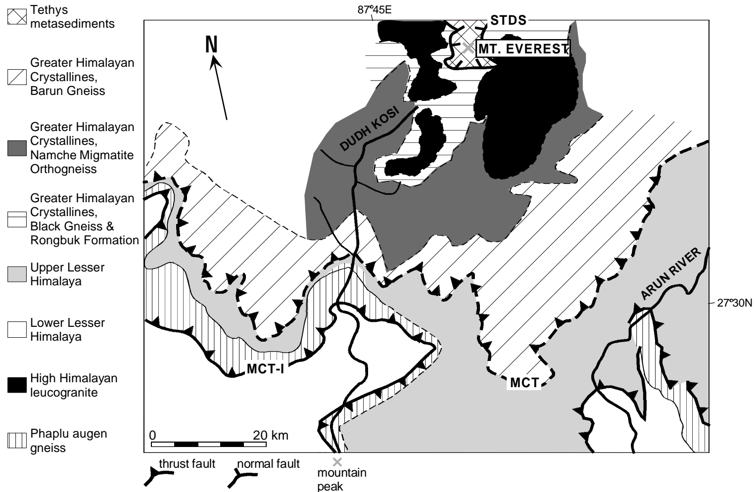
Figure 2.4. Generalized geologic map of eastern Nepal after Lombardo et al. (1993), Akiba et al. (1973), and field interpretations in this dissertation.
