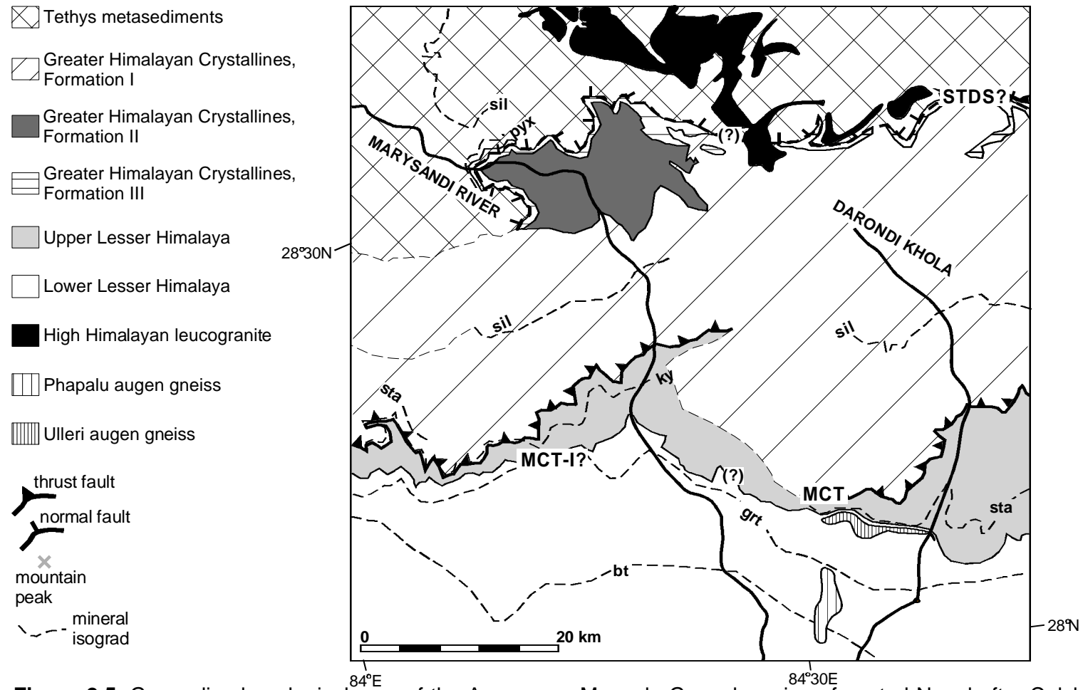
Figure 2.5. Generalized geological map of the Annapurna-Manaslu-Ganesh region of central Nepal after Colchen et al. (1980). Isograds are dashed and labeled: bt= biotite, grt= garnet; ky= kyanite; sta= staurolite; sil= sillimanite; pyx= pyroxene, carbonate lithologies. STDS? = the presence of the South Tibetan Detachment is debated; MCT= Main Central Thrust; MCT-I?= the presence of Arita's (1983) thrust at the base of the MCT shear zone is debated.
