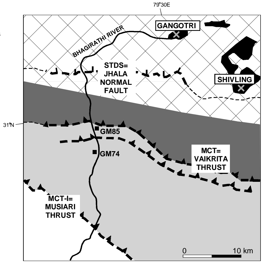
Figure 2.6. Generalized geologic map of the Garhwal Himalaya, India after Metcalfe (1993). No augen gneiss analogous to the Phaplu augen gneiss of eastern Nepal is reported in this area. MCT= Vaikrita Thrust (e.g., Ahmad et al., 2000), and the STDS= Jhala normal fault (e.g., Metcalfe, 1993). Samples GM74 and GM85 after Metcalfe (1993).
